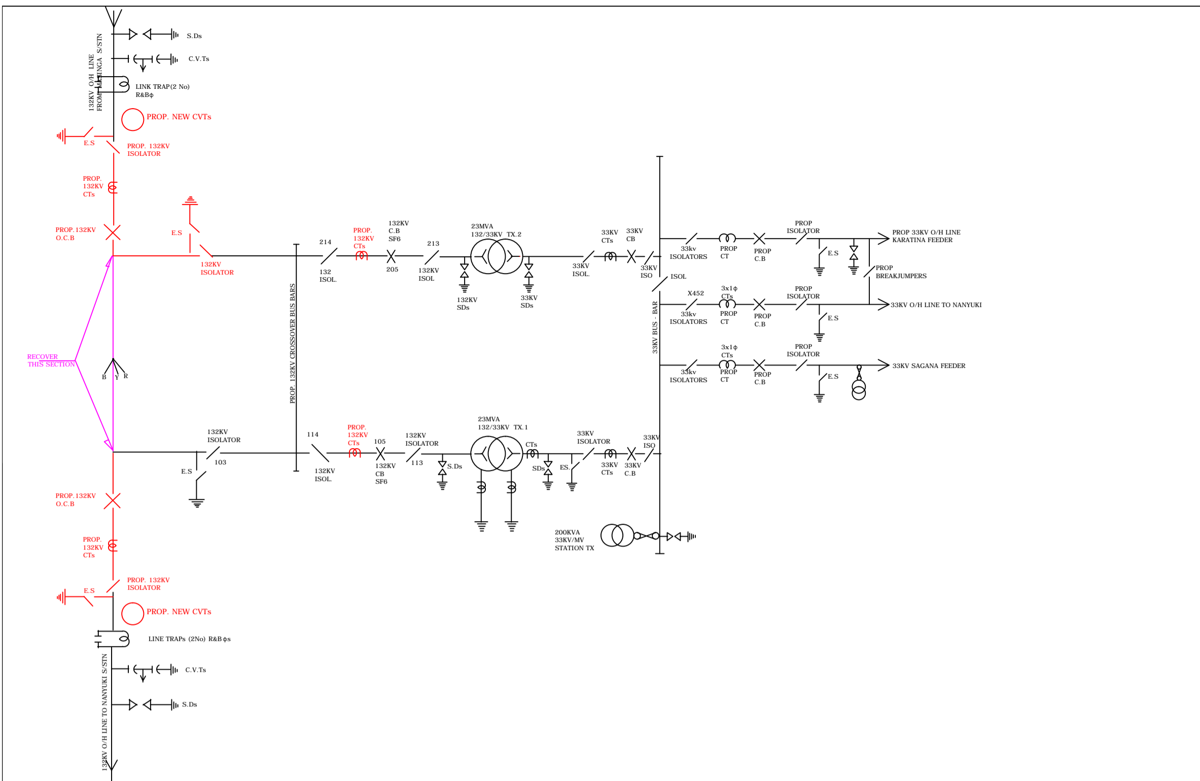
SCHMATIC DIAGRAM
