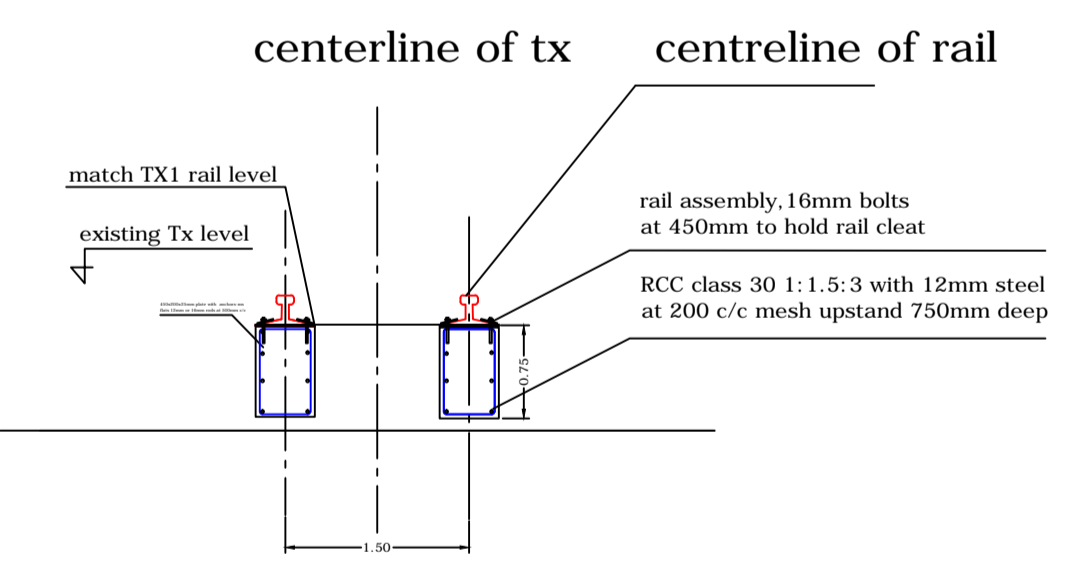
section x-x
