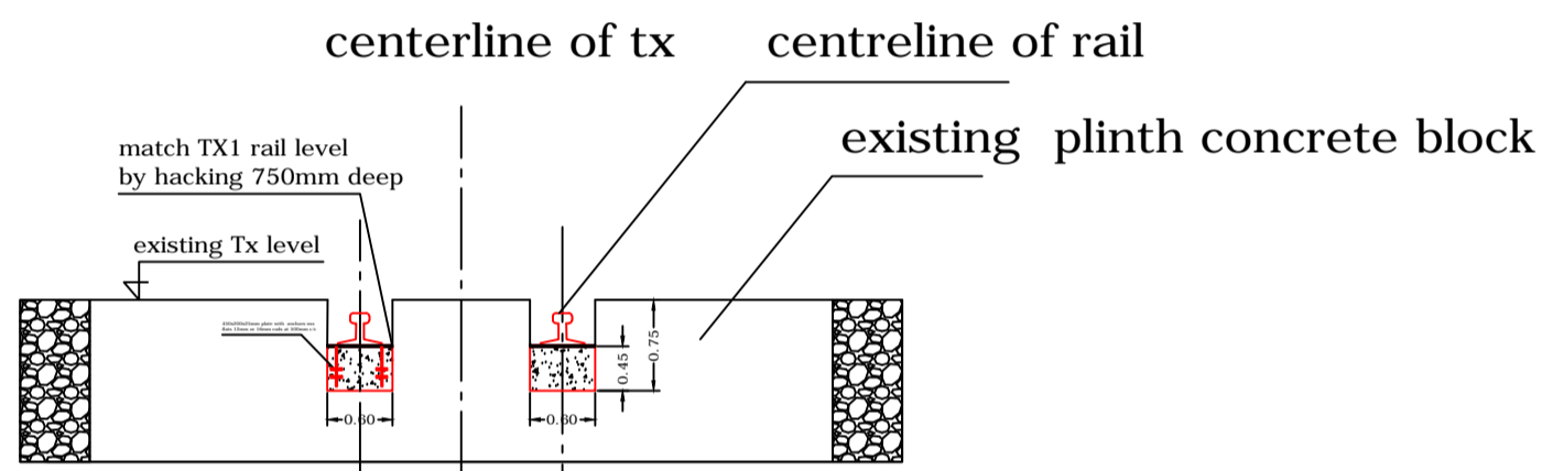
section at existing plinth
